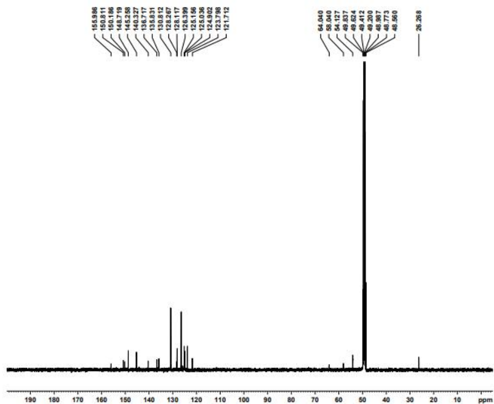
Figure S6. ^{13}\text{C} NMR spectrum of TTVP.
